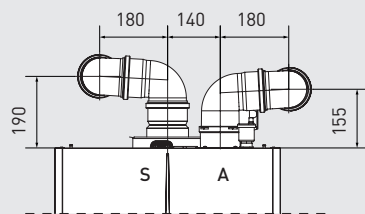
Separator kit distances Ø 100/100
