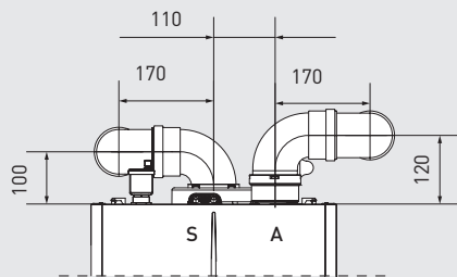
Separator kit distances Ø 80/80
